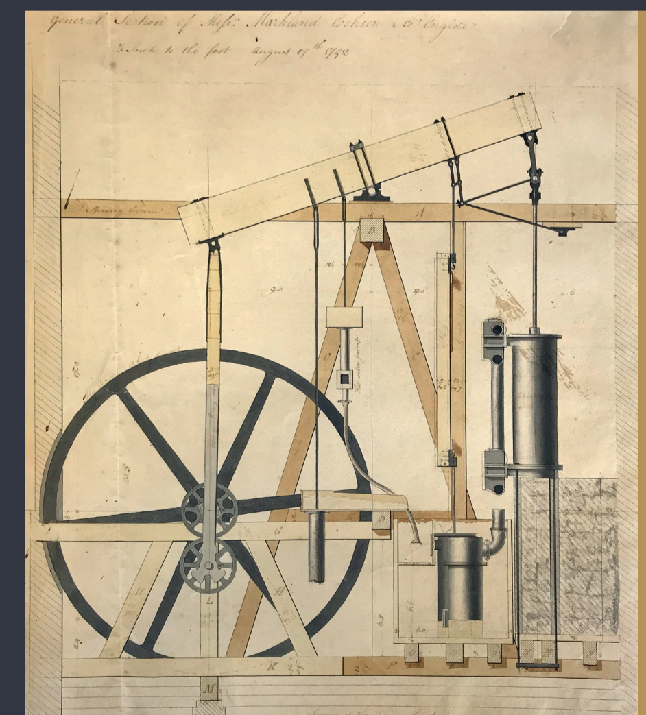
Boulton & Watt rotary steam engine design, 1792 © Birmingham Libraries
