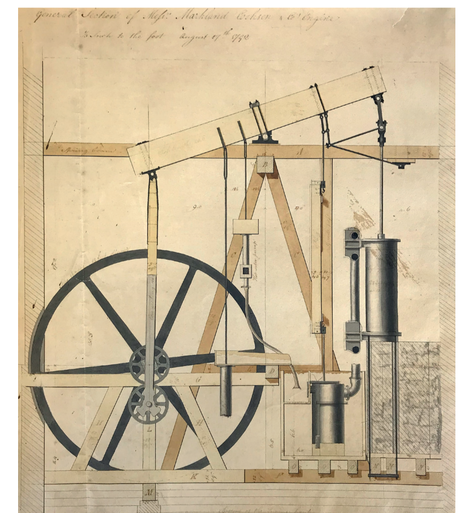
Boulton & Watt rotary steam engine design, 1792
