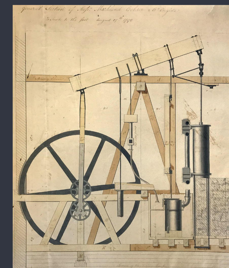
Boulton & Watt rotary steam engine design, 1792 © Birmingham Libraries
