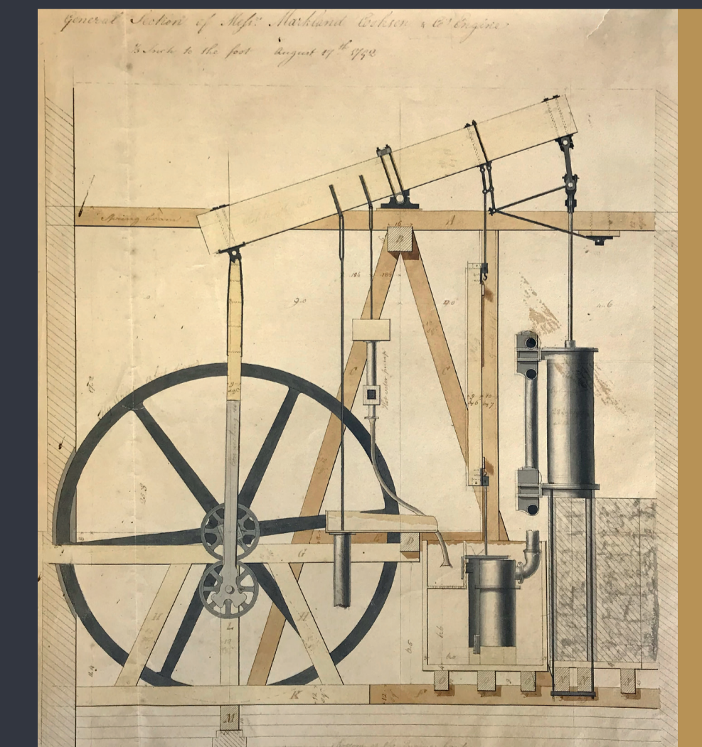
Boulton & Watt rotary steam engine design, 1792 © Birmingham Libraries
